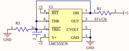
Astable Clock Module
